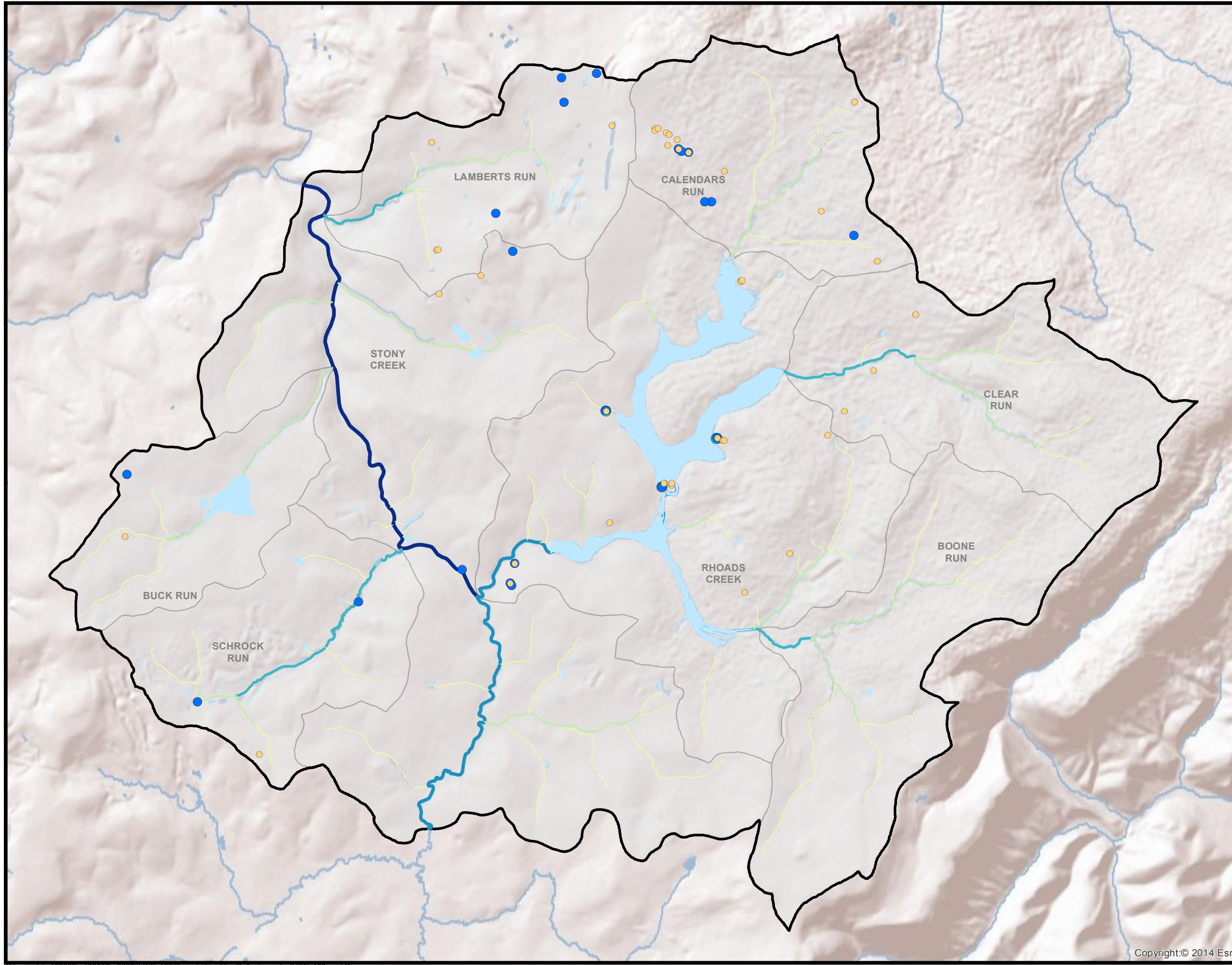
Figure 4 Hydrogeologic Model Elements Indian Lake Borough Waterworks PWSID# 4560025 Somerset County, PA Source Water Protection Technical Assistance Program
